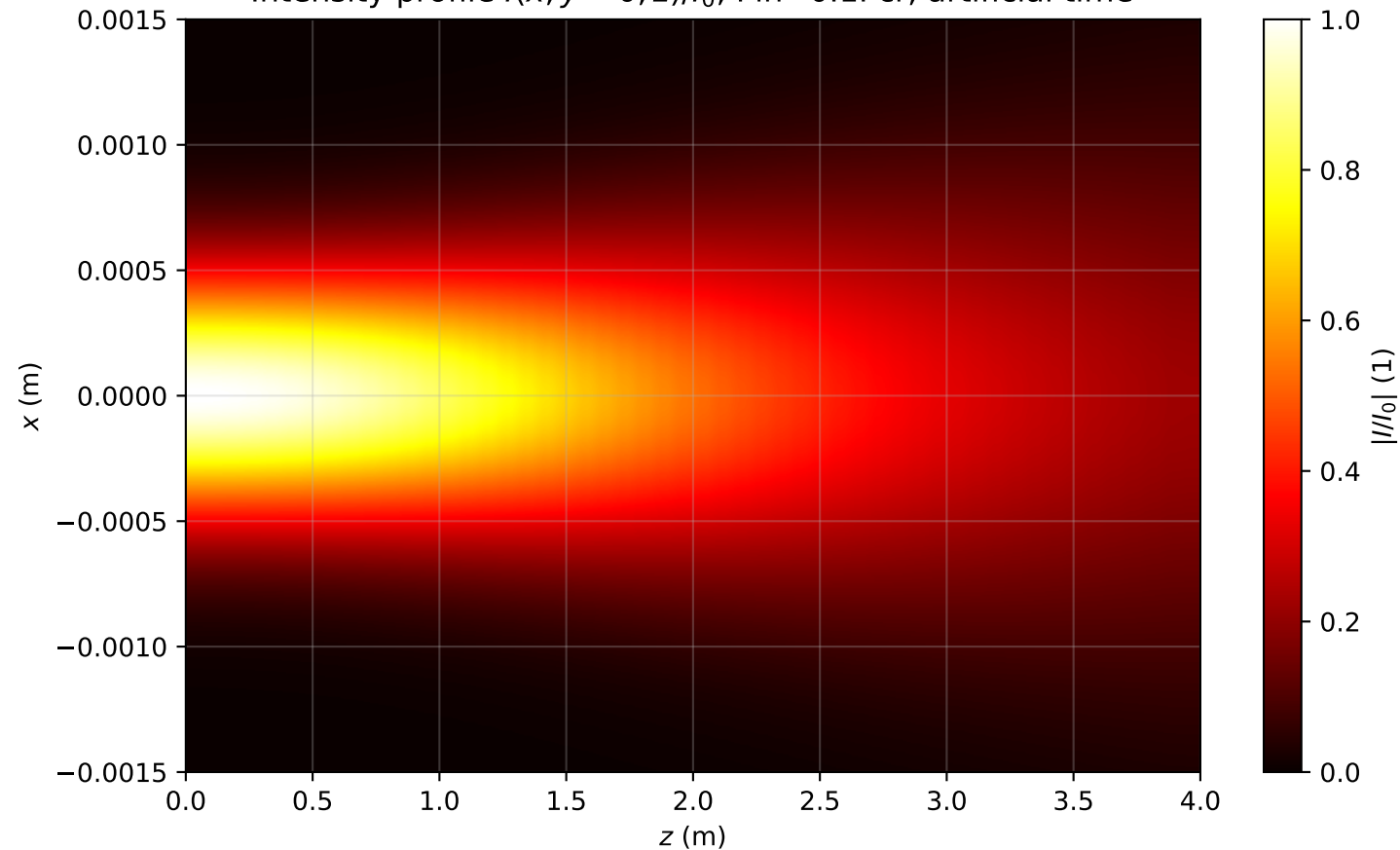
Intensity profile I(x, y = 0, z)/I_0 , P_{in}=0.1P_{cr} , artificial time
